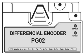
SSI800-PG02/Differential Mode Incremental Encoder
